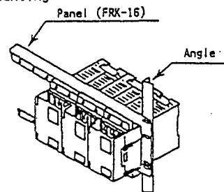
Fig.1 Rack Mounting
