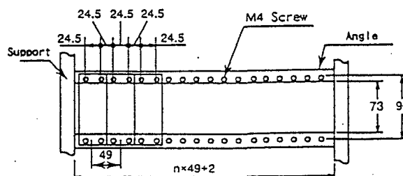
Fig.5 Angle Mounting Dimension
